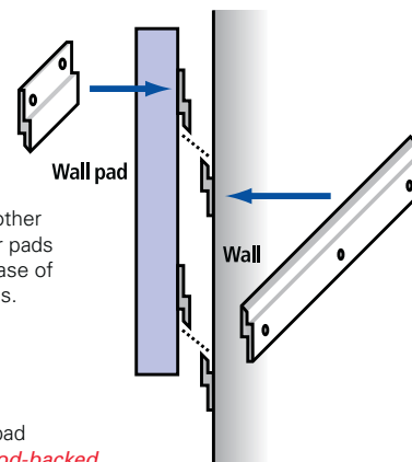
Z-Clip/Z-Bar systems: Side view
